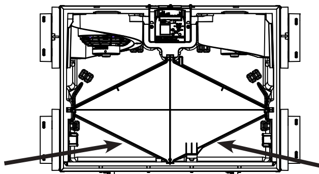
MERV8 FILTER REPLACEMENT
